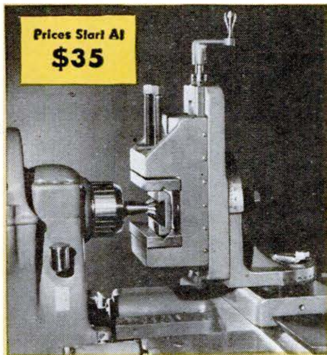
Milling and Keyway Cutting Attachment
